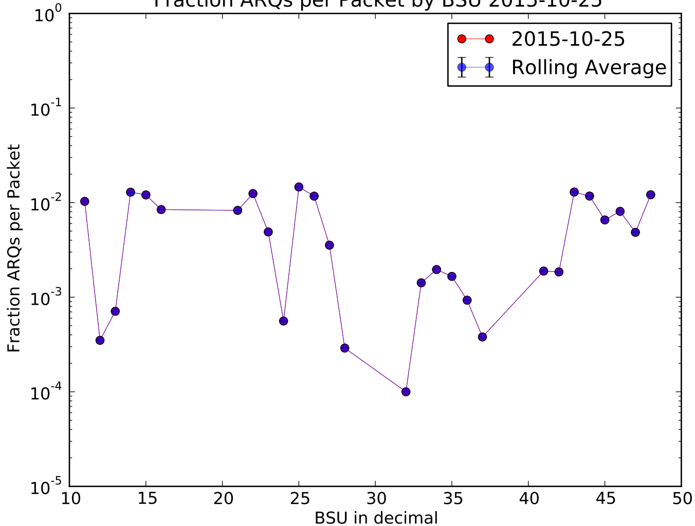
Fraction ARQs per Packet by BSU 2015-10-25
