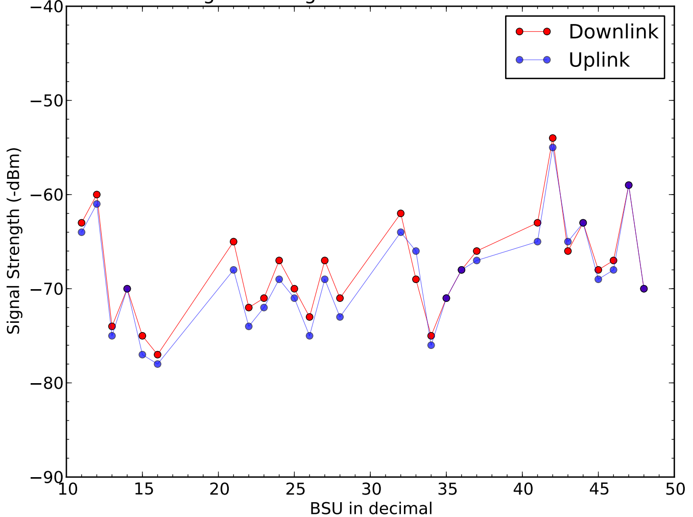
Signal Strength of BSU on 2015-10-25
