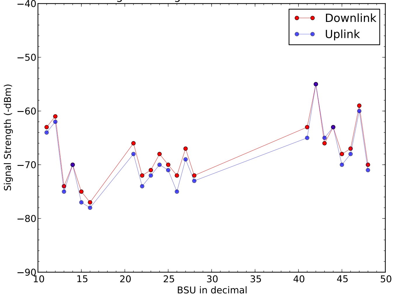
Signal Strength of BSU on 2015-11-02
