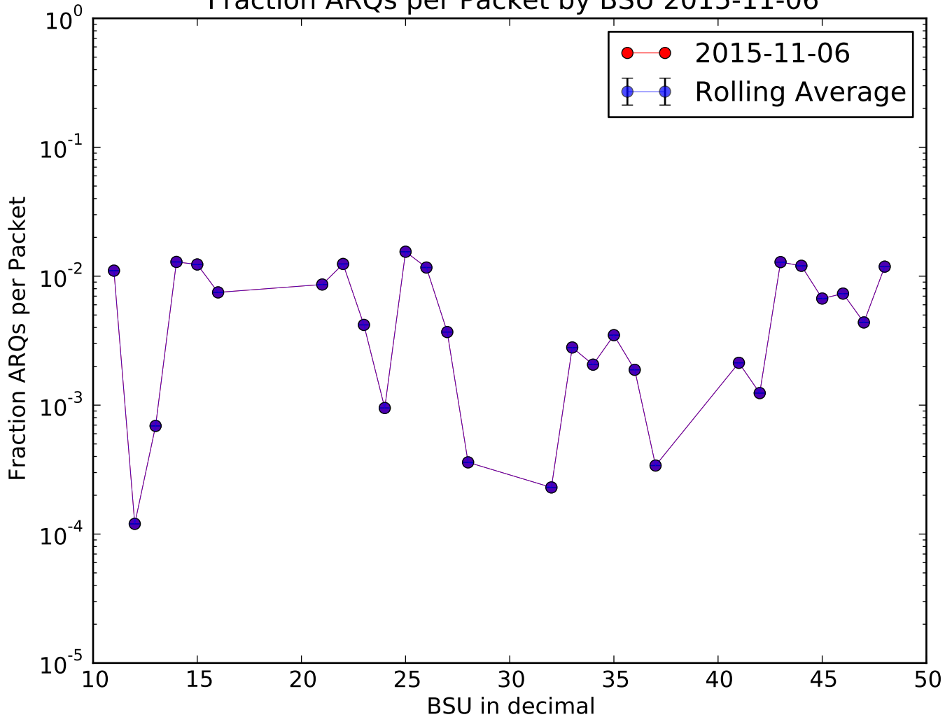
Fraction ARQs per Packet by BSU 2015-11-06
