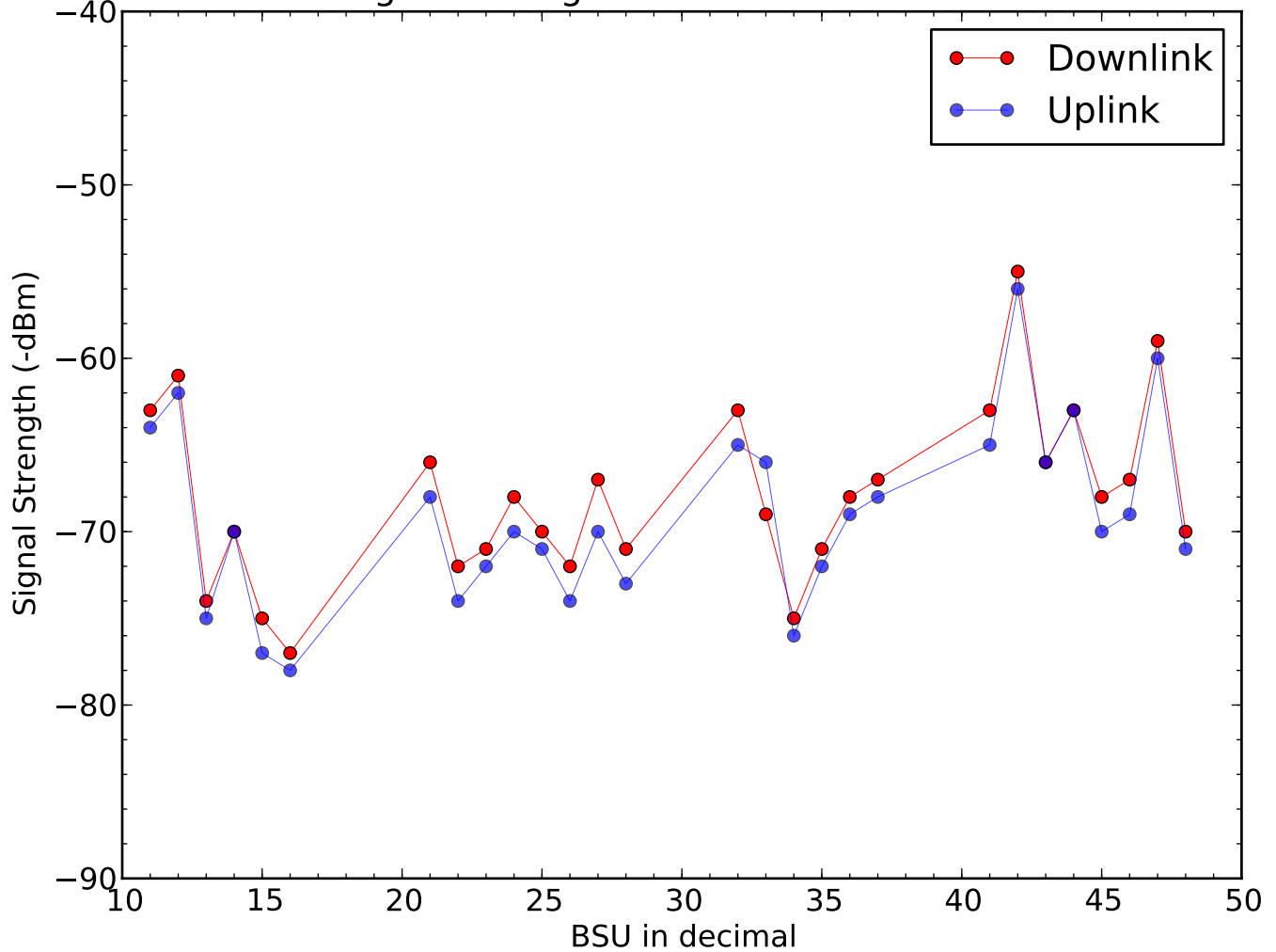
Signal Strength of BSU on 2015-11-12
