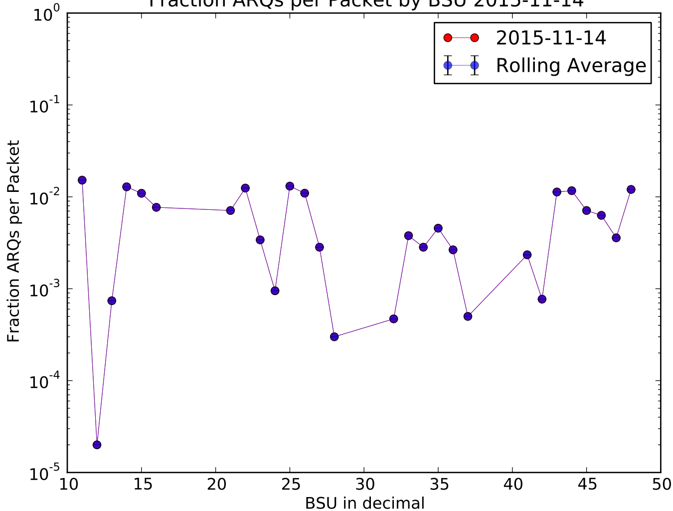
Fraction ARQs per Packet by BSU 2015-11-14
