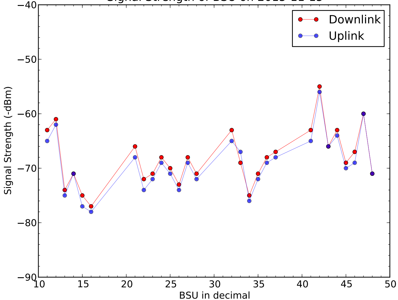
Signal Strength of BSU on 2015-11-15
