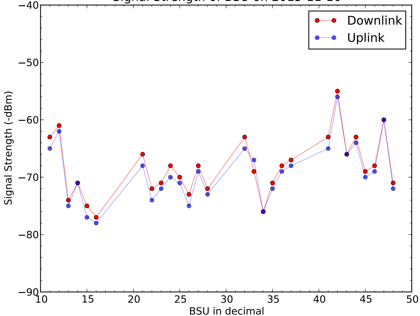
Signal Strength of BSU on 2015-11-16
