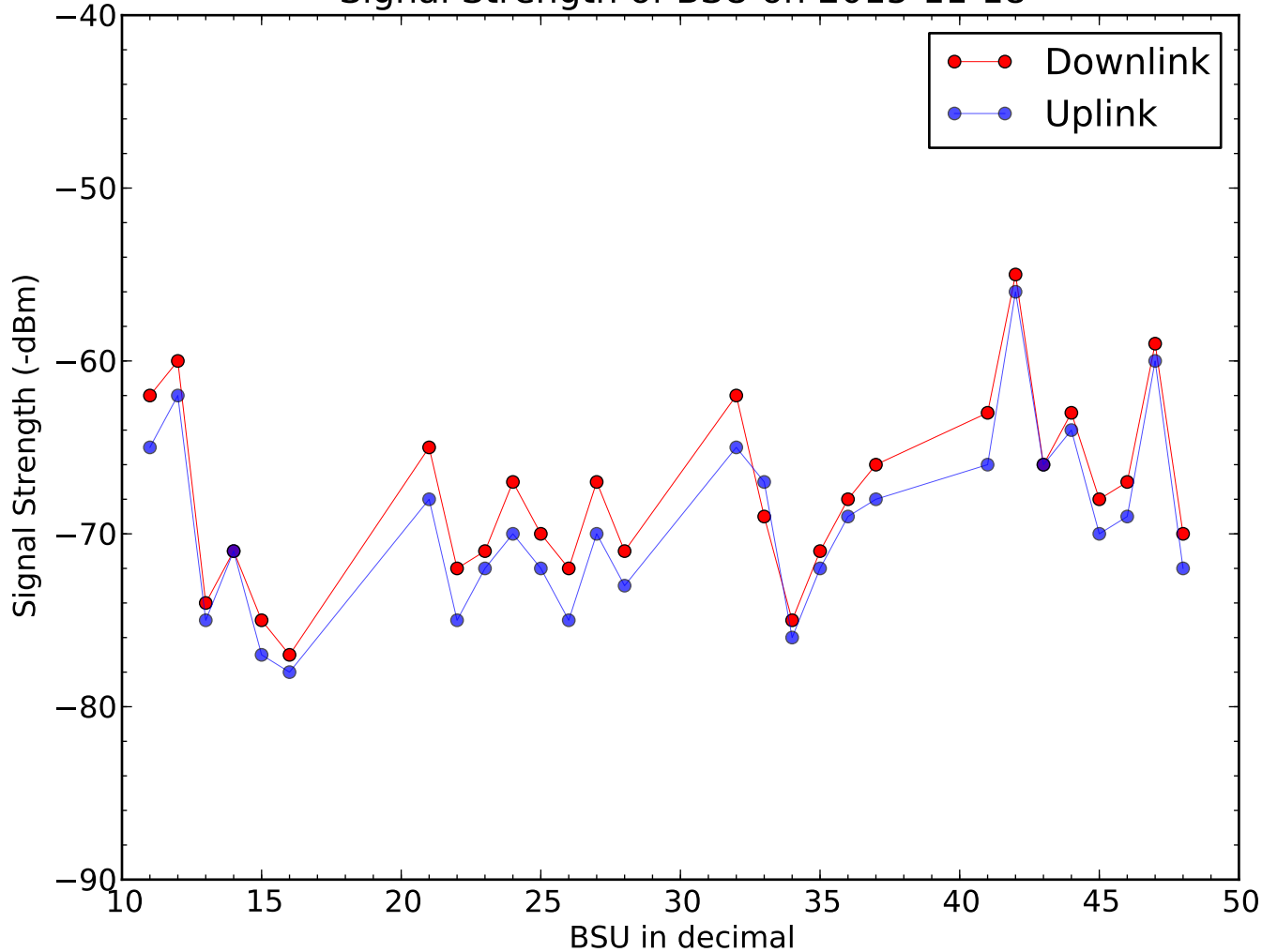
Signal Strength of BSU on 2015-11-18
