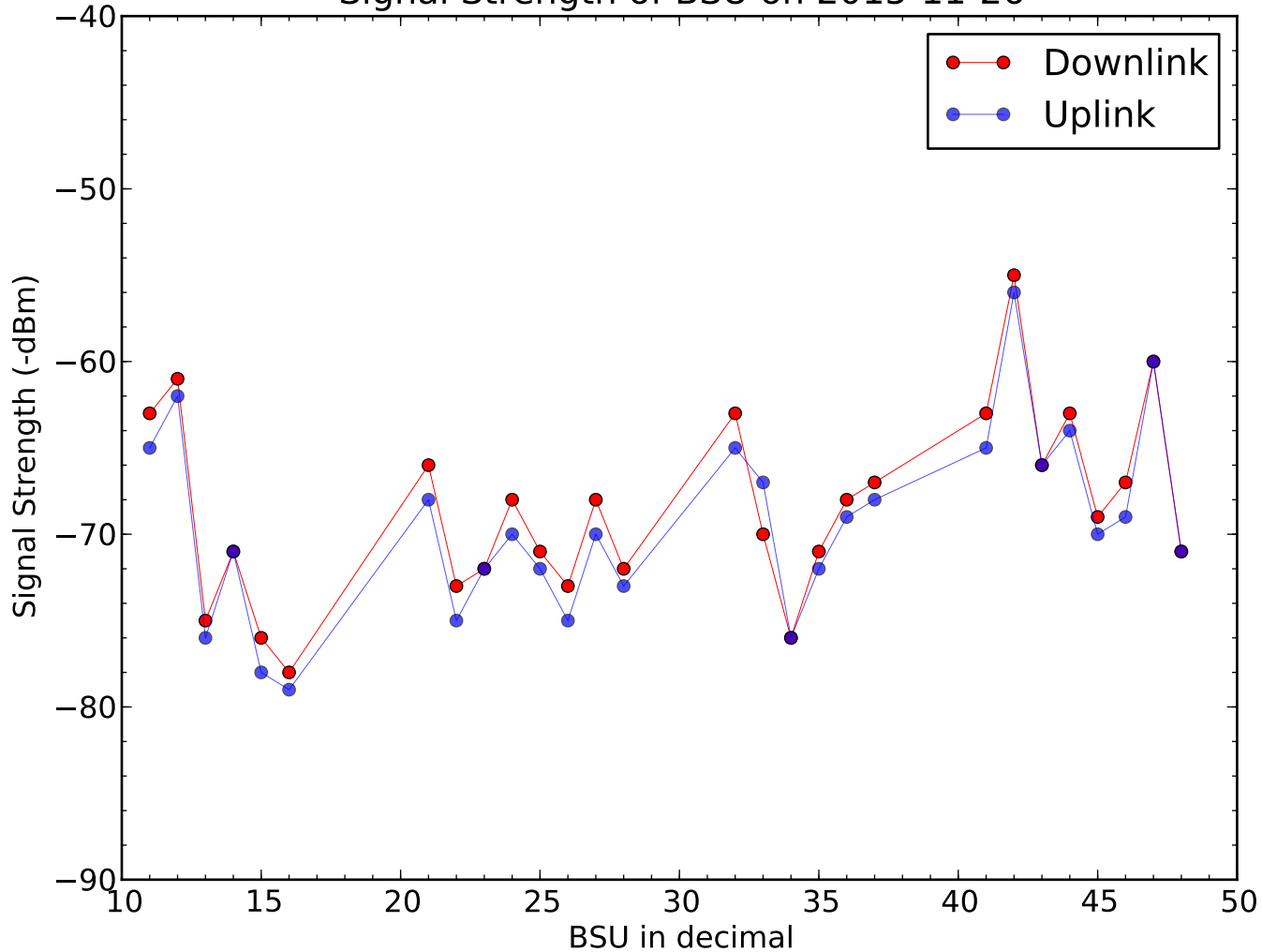
Signal Strength of BSU on 2015-11-26
