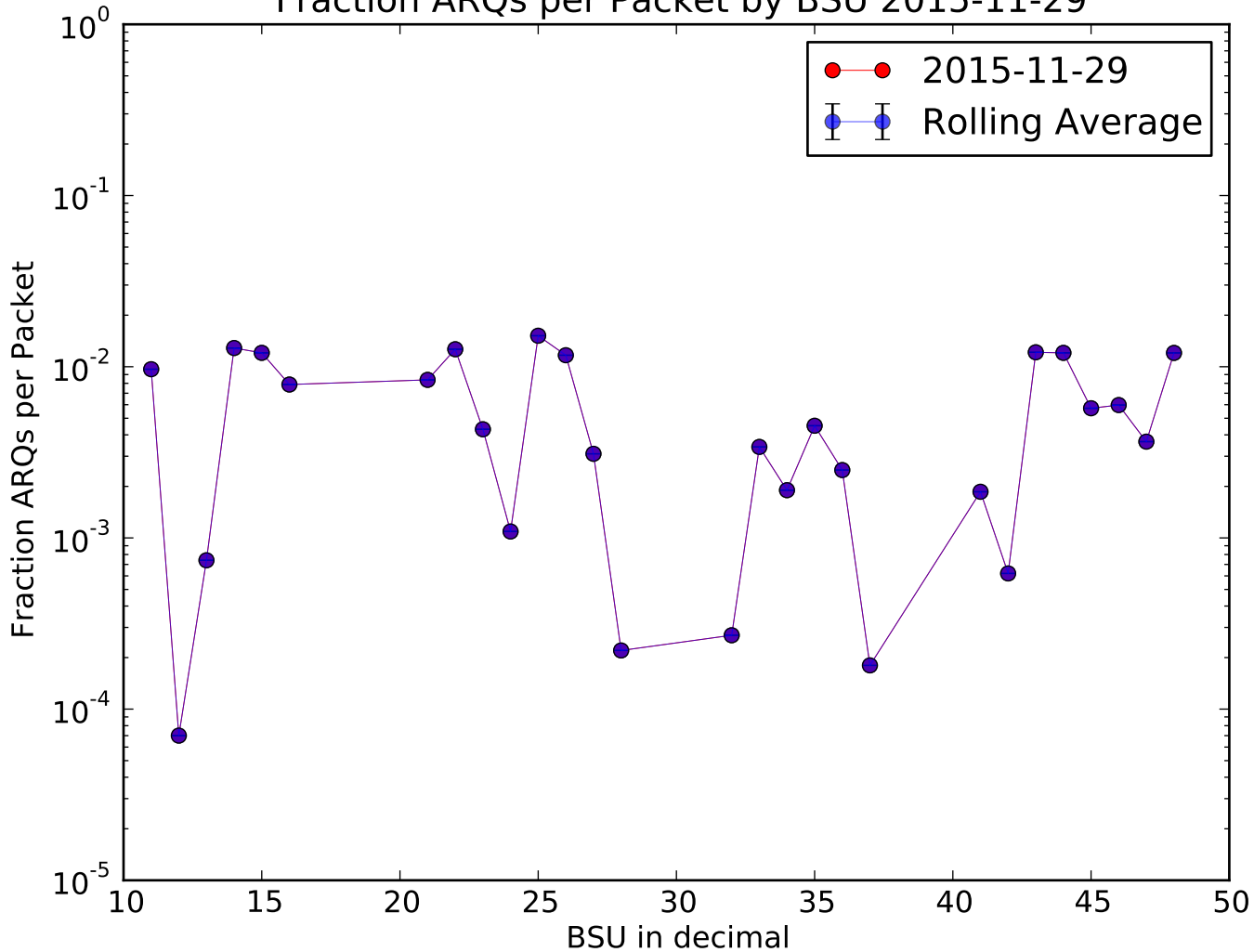
Fraction ARQs per Packet by BSU 2015-11-29
