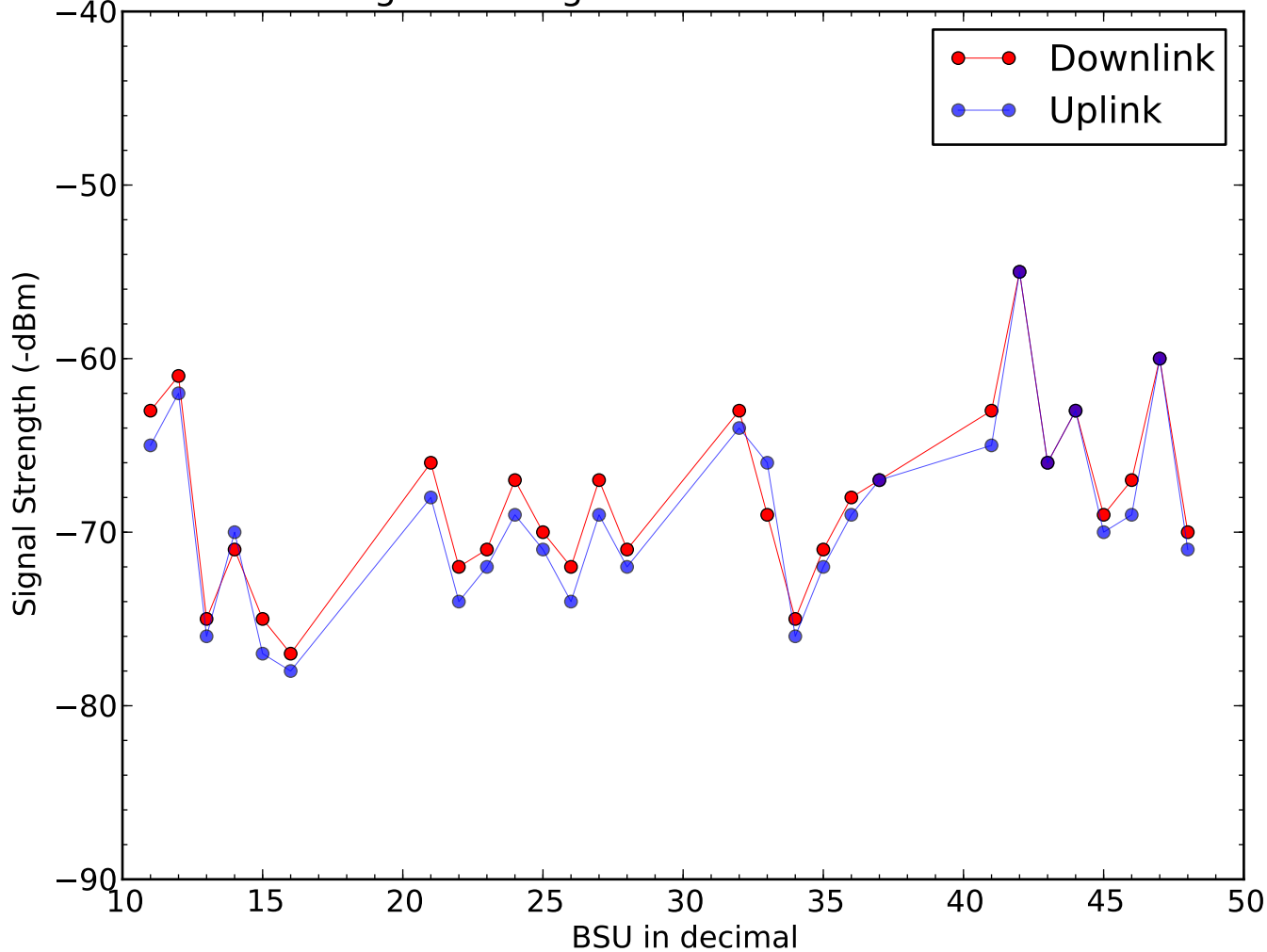
Signal Strength of BSU on 2015-11-29
