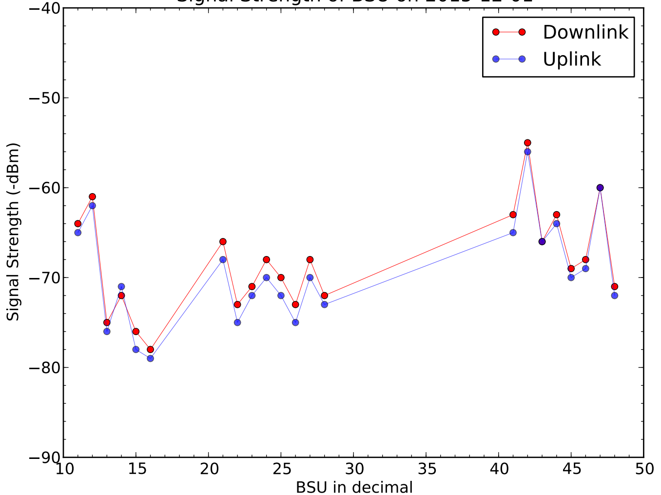
Signal Strength of BSU on 2015-12-01
