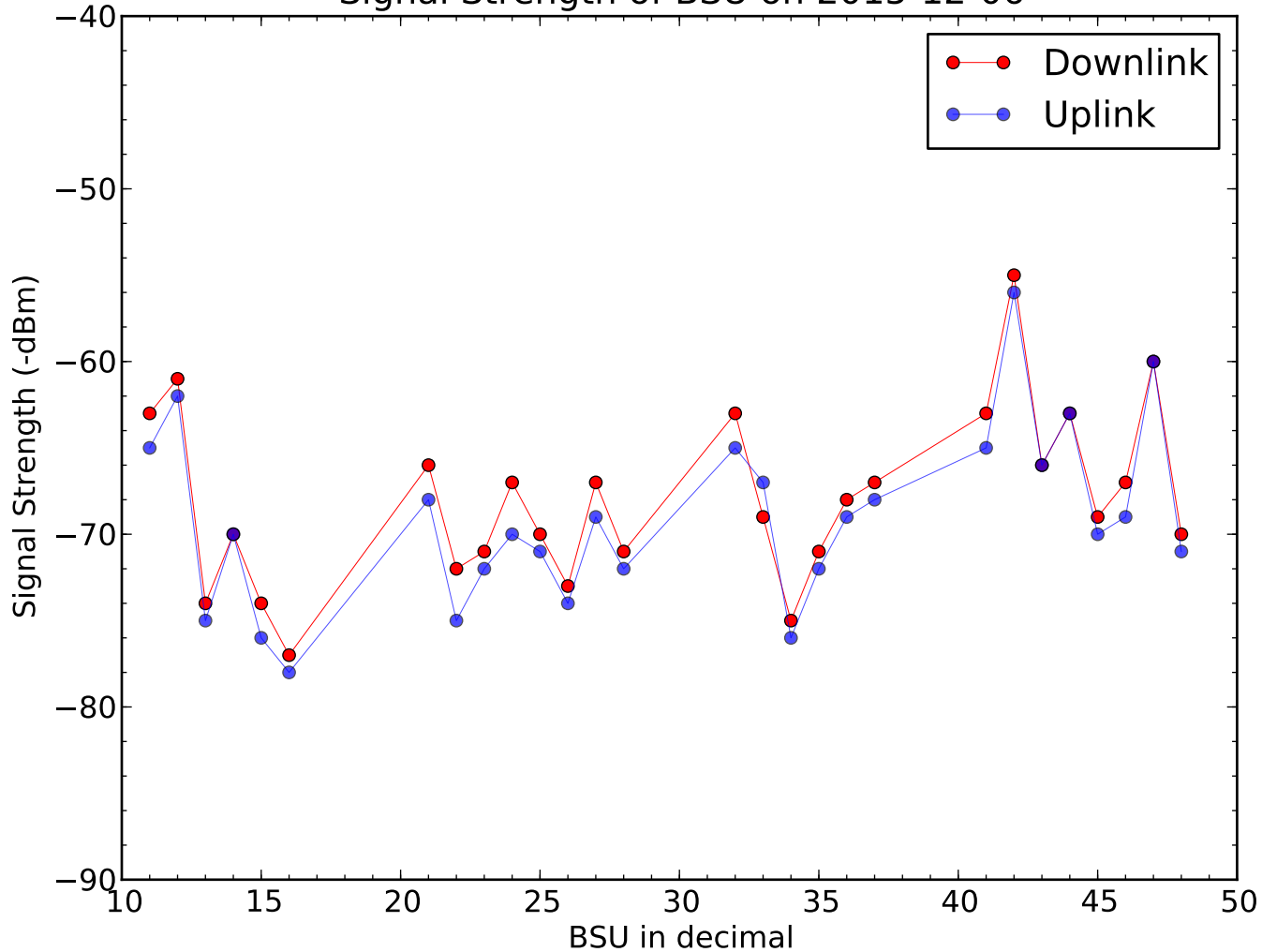
Signal Strength of BSU on 2015-12-06
