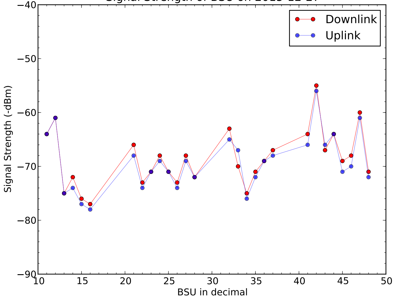
Signal Strength of BSU on 2015-12-27
