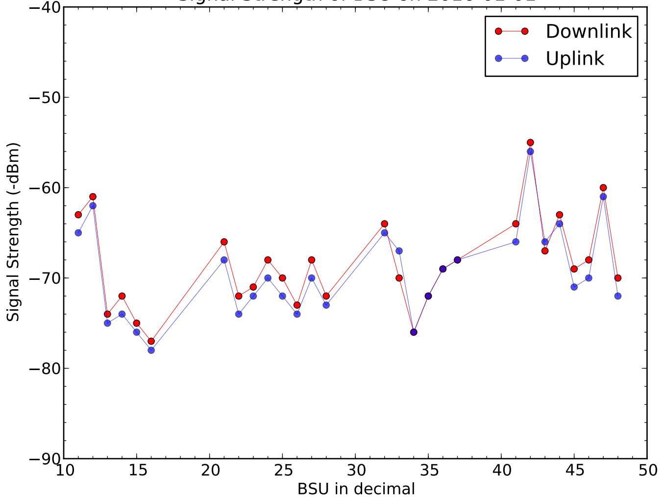
Signal Strength of BSU on 2016-01-01
