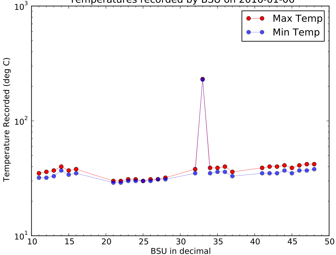
Temperatures recorded by BSU on 2016-01-06
