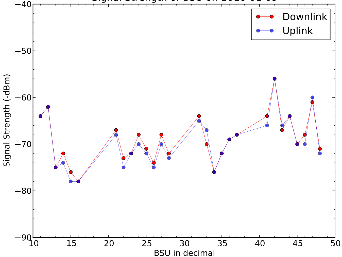
Signal Strength of BSU on 2016-01-09
