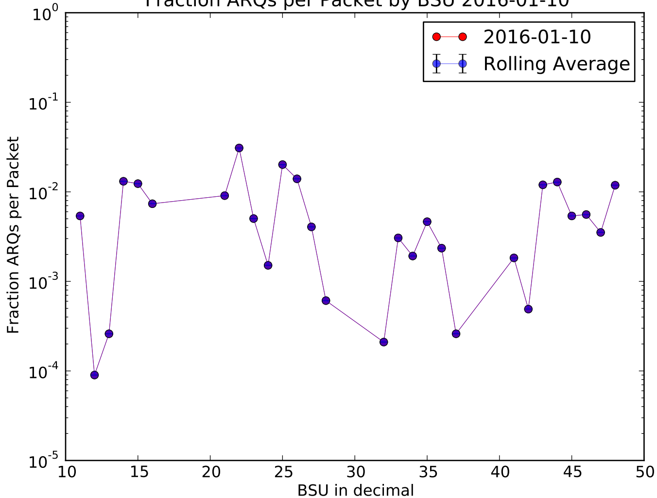
Fraction ARQs per Packet by BSU 2016-01-10
