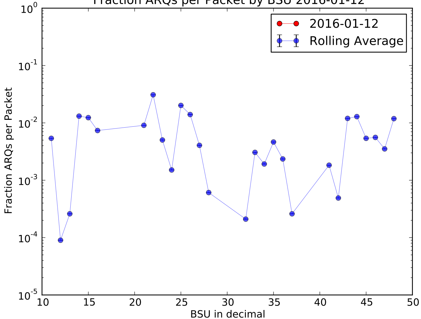
Fraction ARQs per Packet by BSU 2016-01-12
