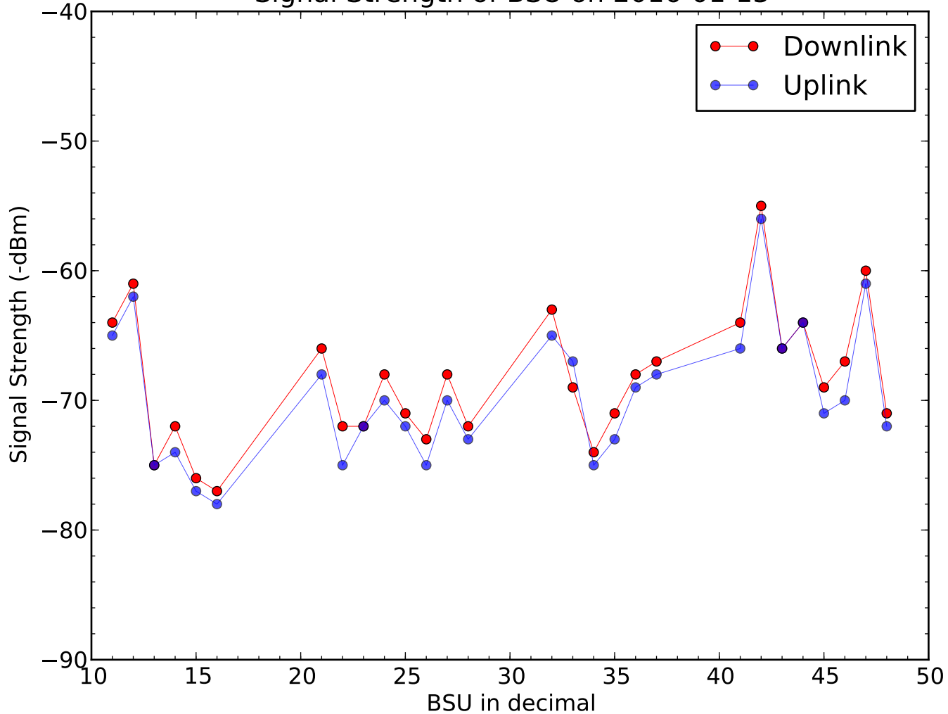
Signal Strength of BSU on 2016-01-13
