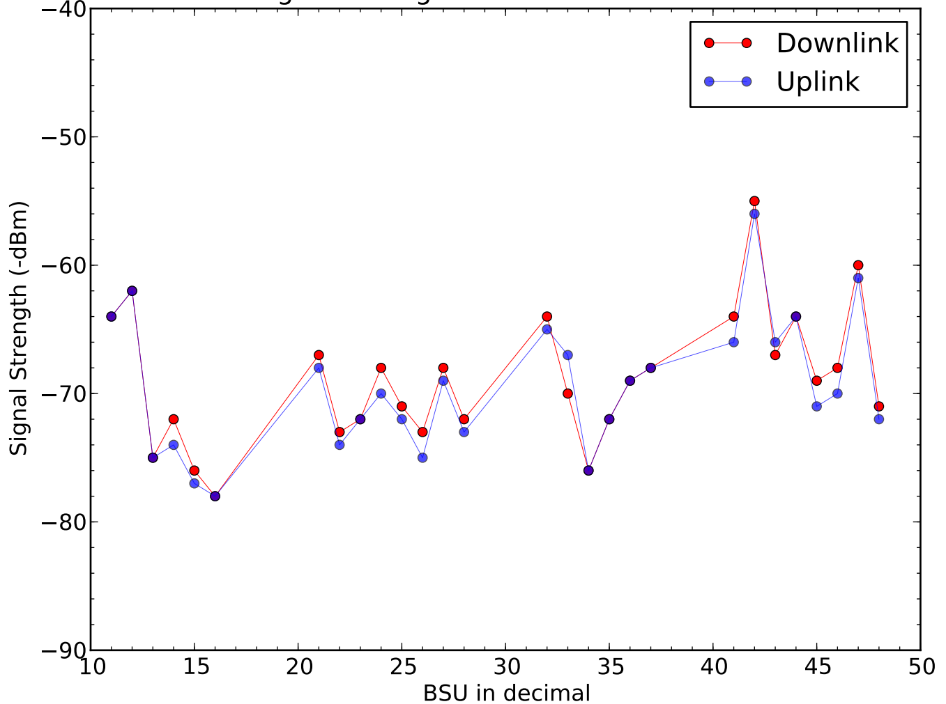
Signal Strength of BSU on 2016-01-15
