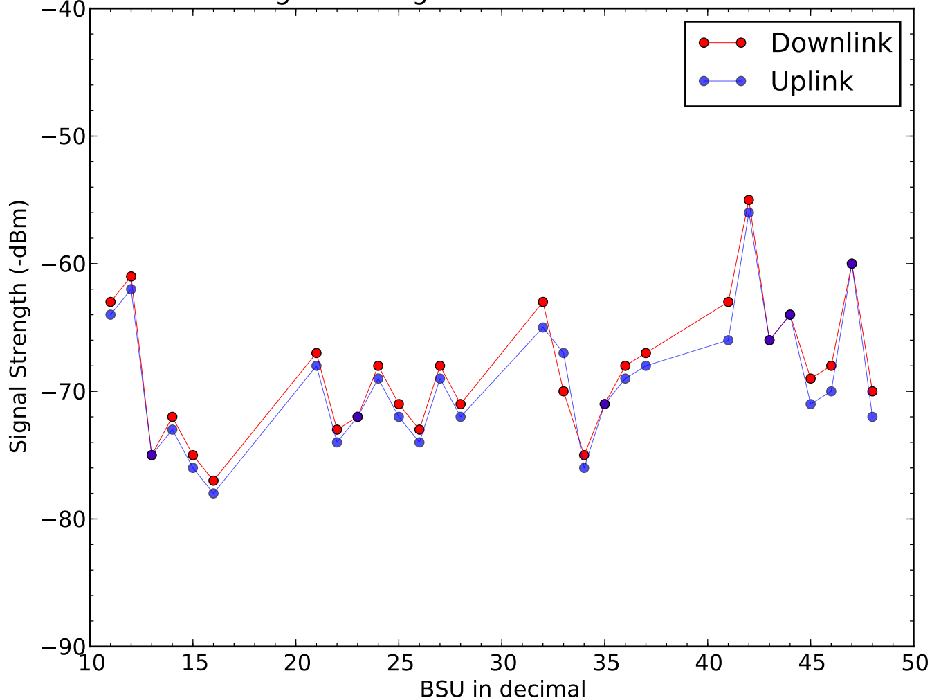
Signal Strength of BSU on 2016-01-16
