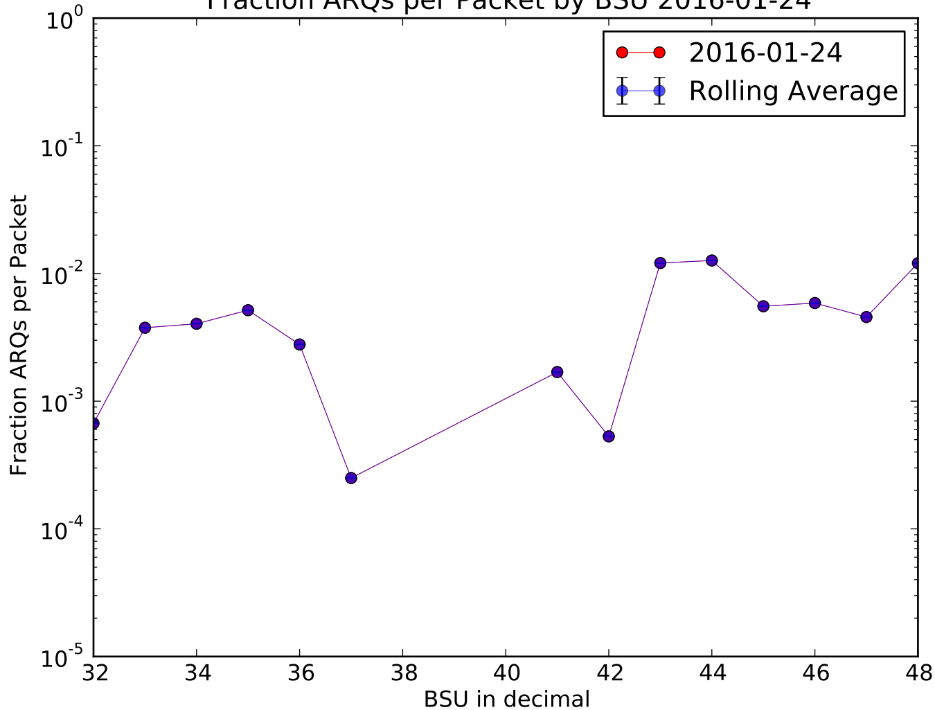
Fraction ARQs per Packet by BSU 2016-01-24
