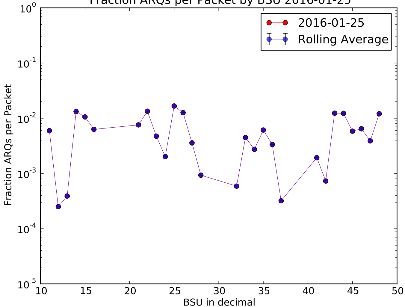
Fraction ARQs per Packet by BSU 2016-01-25
