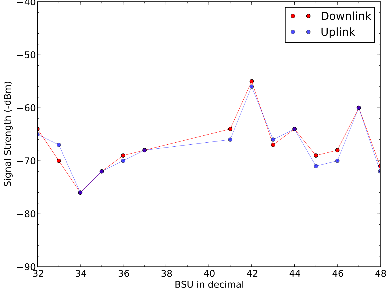
Signal Strength of BSU on 2016-01-30
