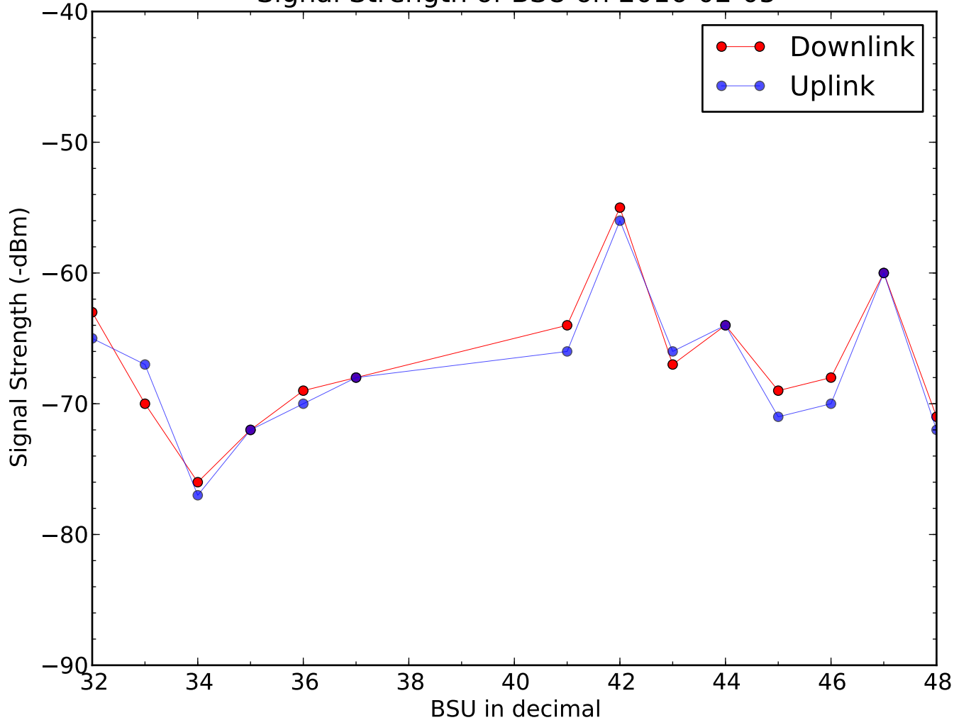
Signal Strength of BSU on 2016-02-05
