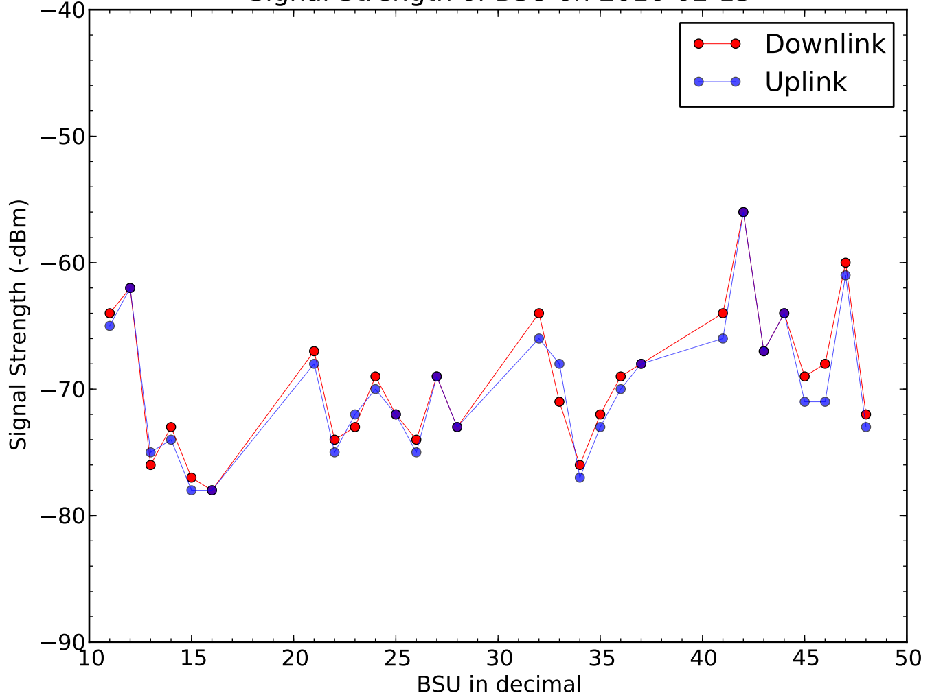
Signal Strength of BSU on 2016-02-13
