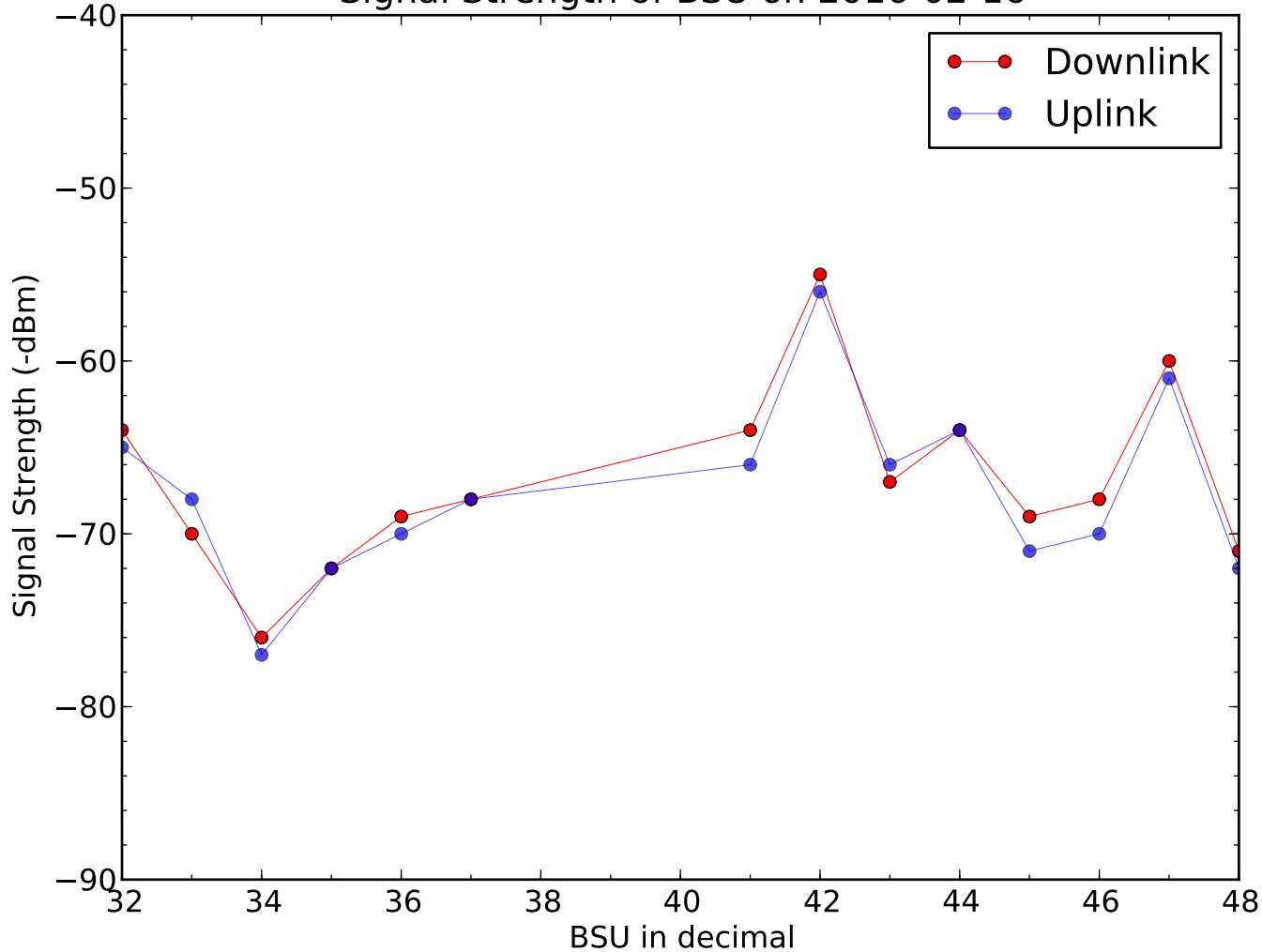
Signal Strength of BSU on 2016-02-16
