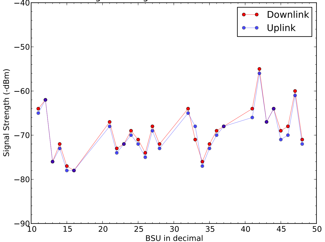
Signal Strength of BSU on 2016-02-23
