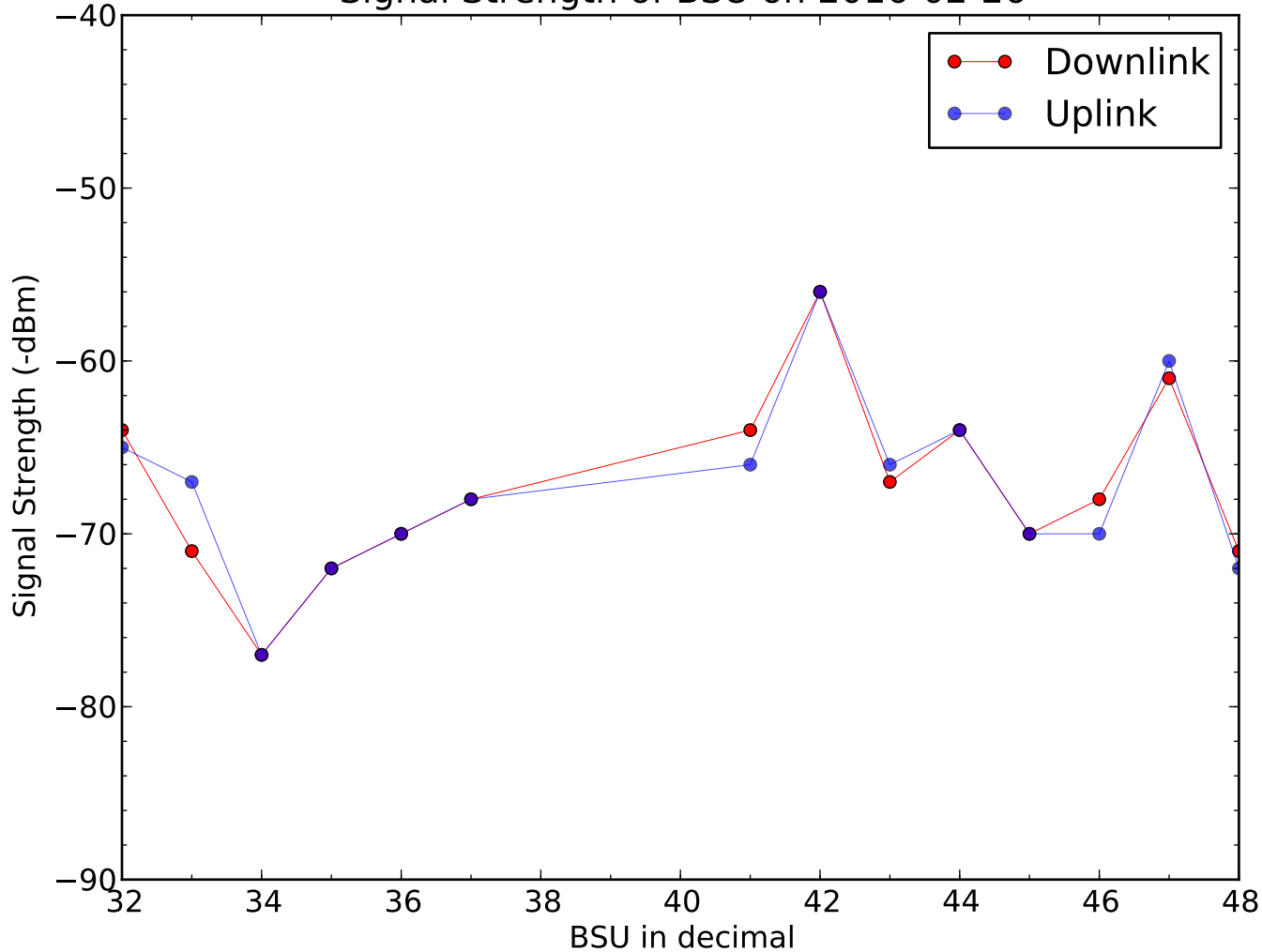
Signal Strength of BSU on 2016-02-26
