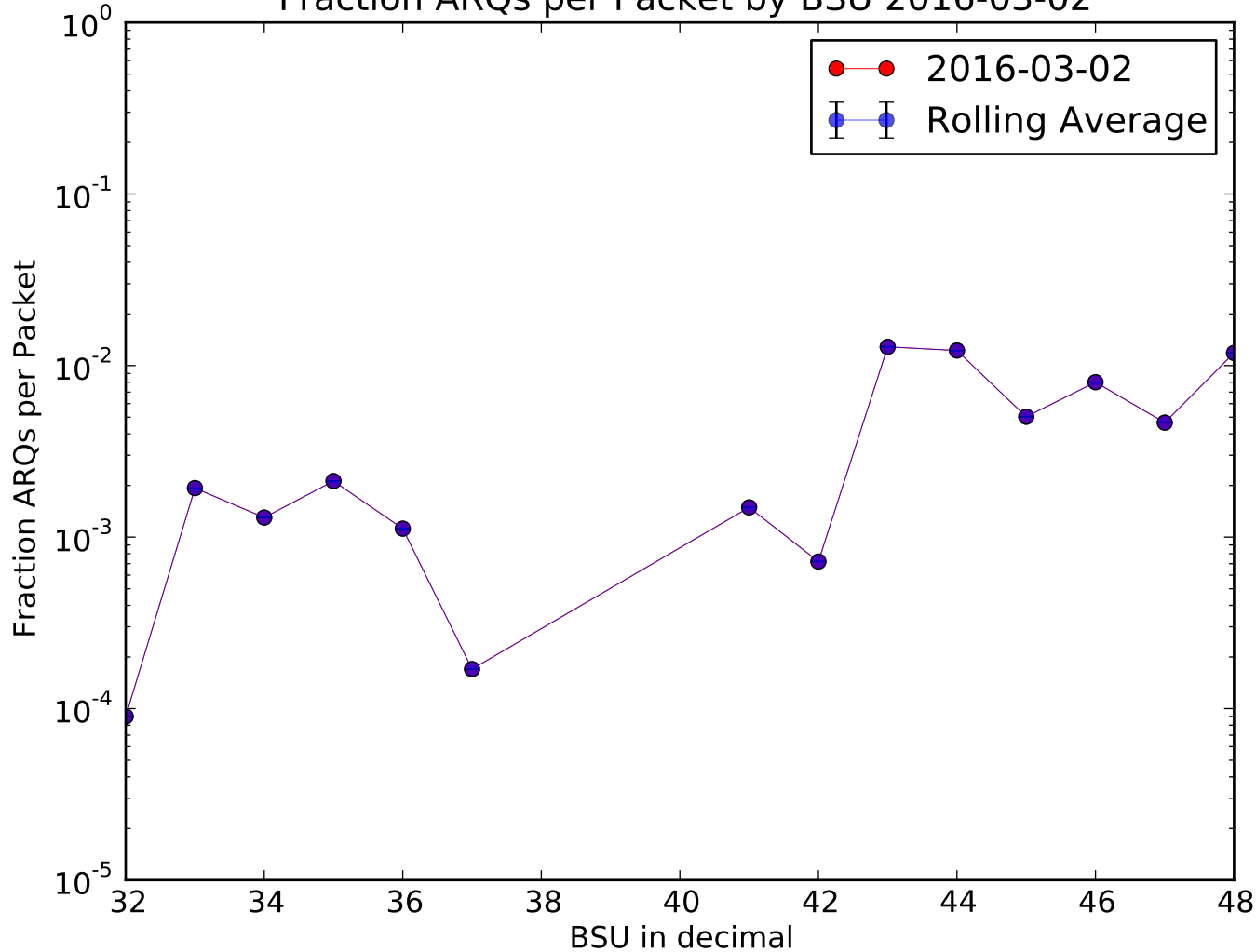
Fraction ARQs per Packet by BSU 2016-03-02
