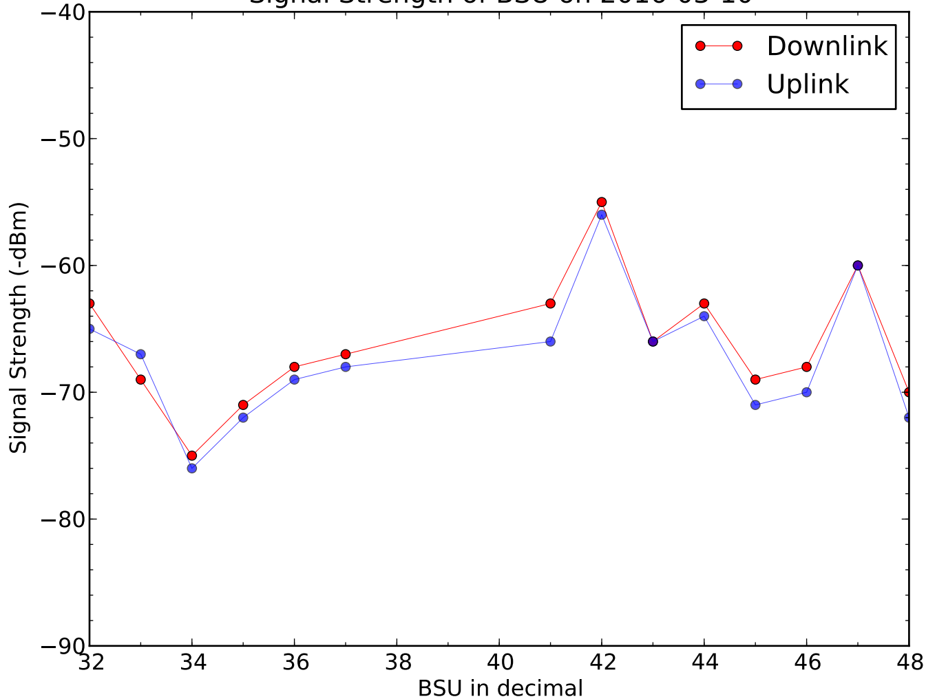
Signal Strength of BSU on 2016-03-10
