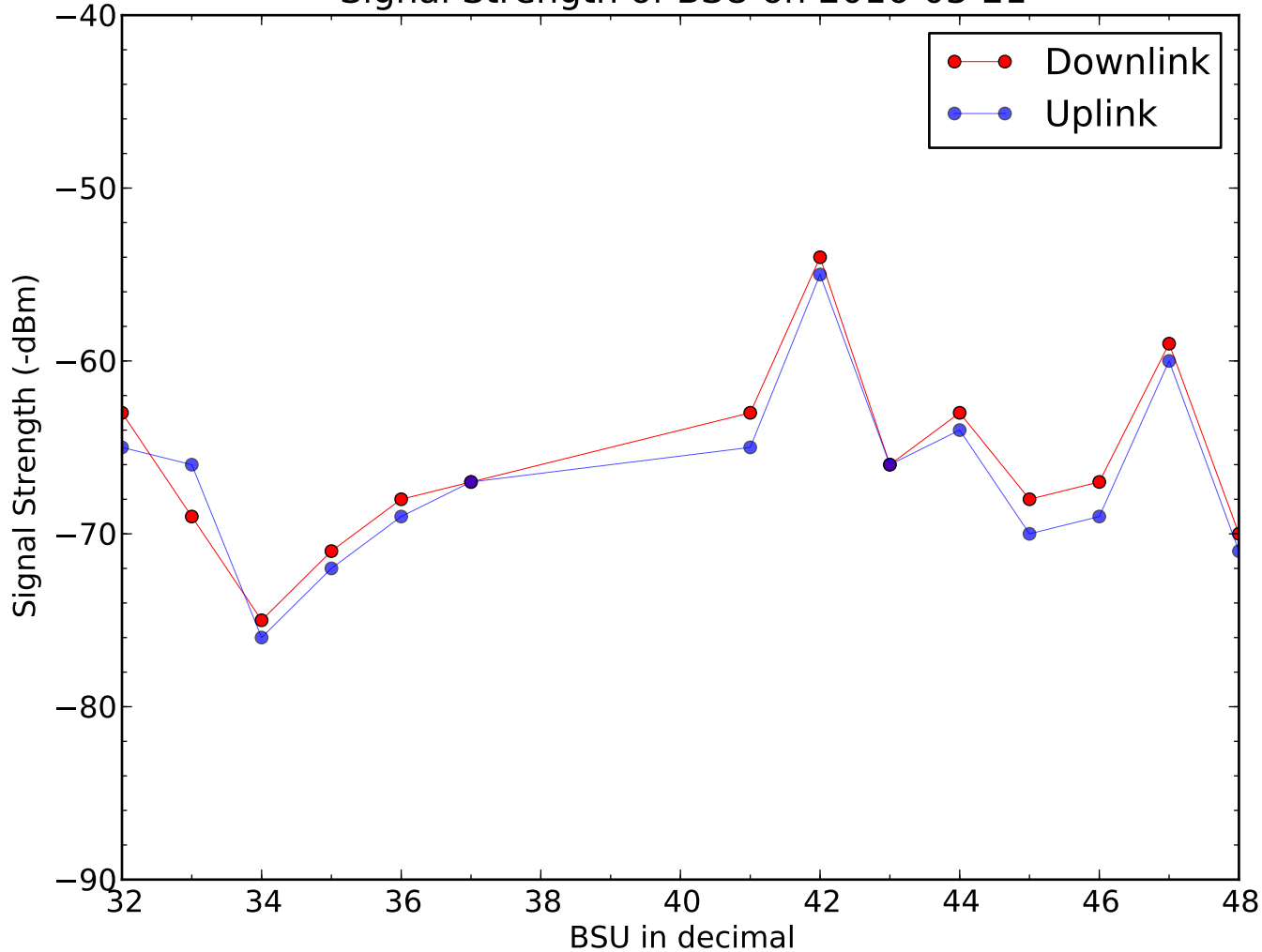
Signal Strength of BSU on 2016-03-21
