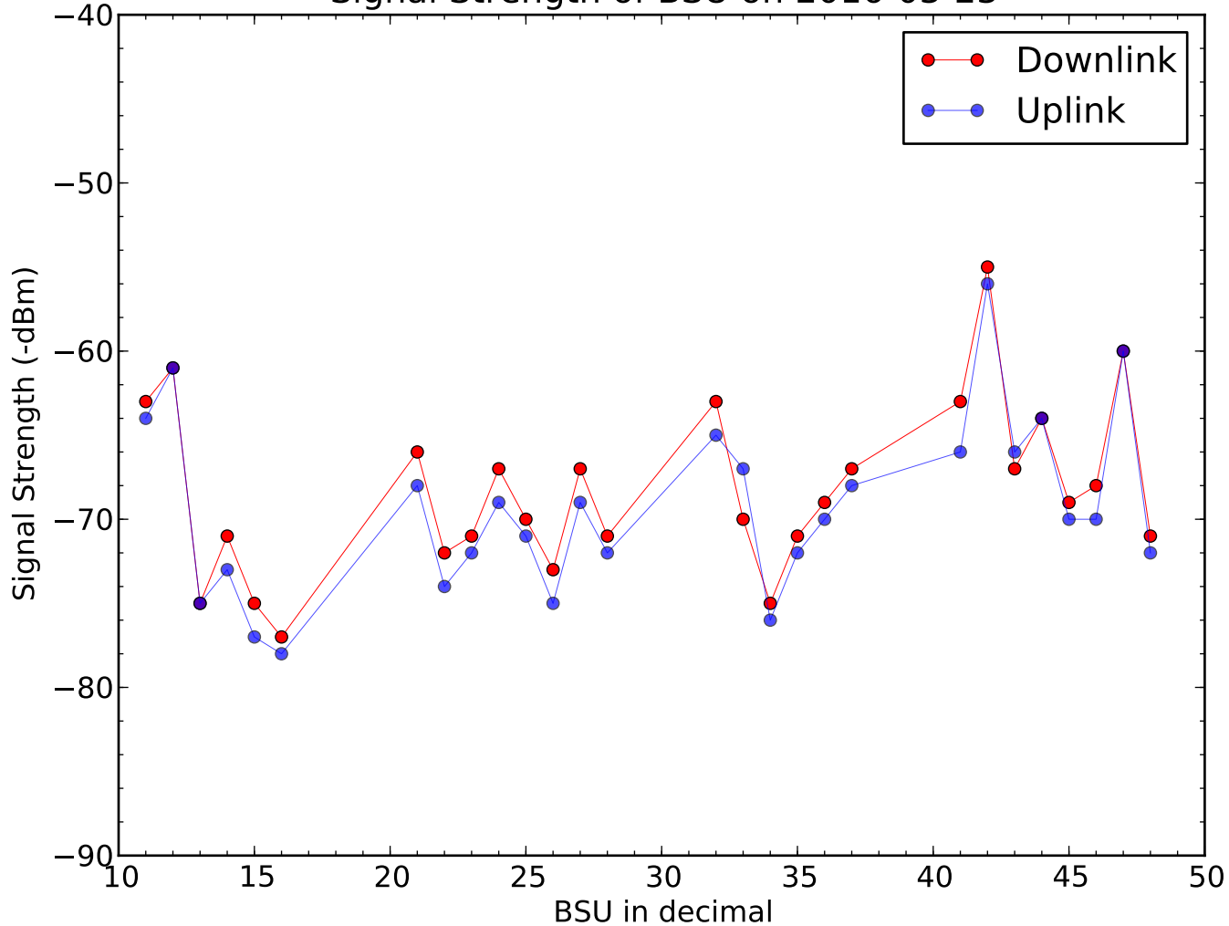
Signal Strength of BSU on 2016-03-23
