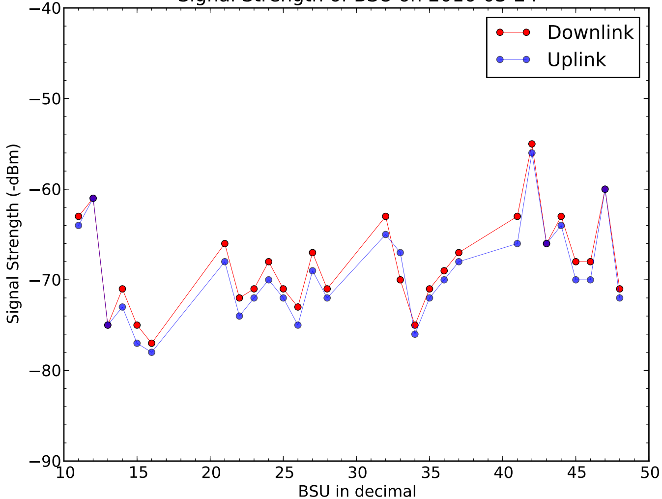
Signal Strength of BSU on 2016-03-24
