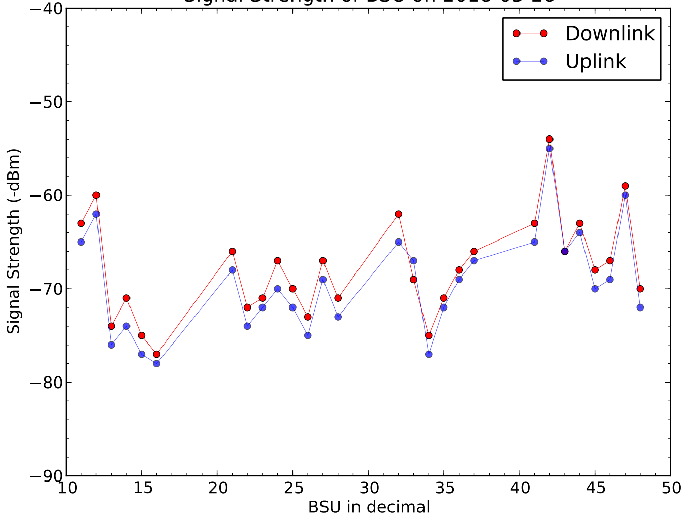
Signal Strength of BSU on 2016-03-26
