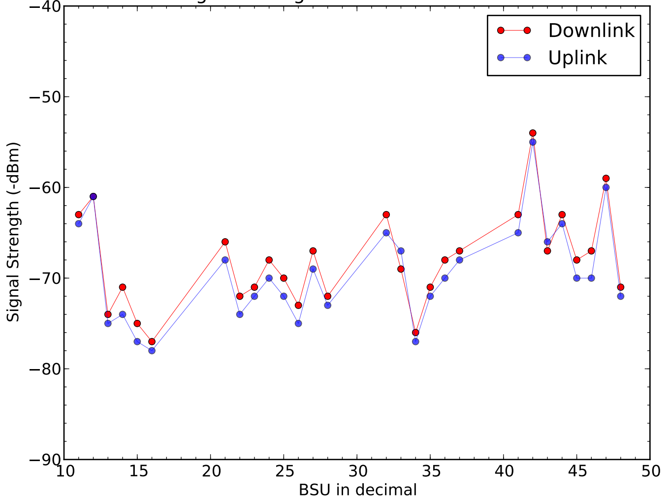
Signal Strength of BSU on 2016-04-02
