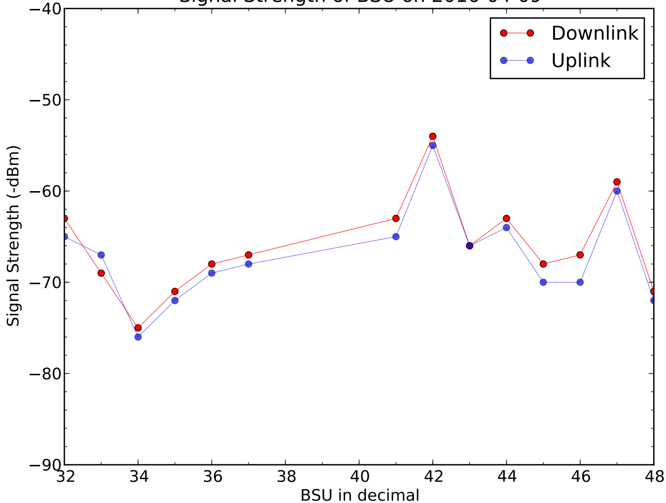
Signal Strength of BSU on 2016-04-09
