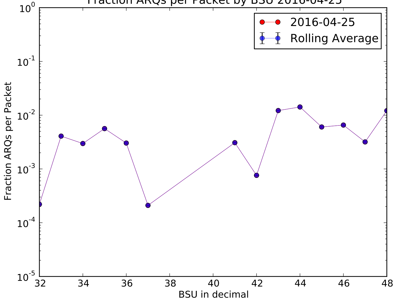
Fraction ARQs per Packet by BSU 2016-04-25
