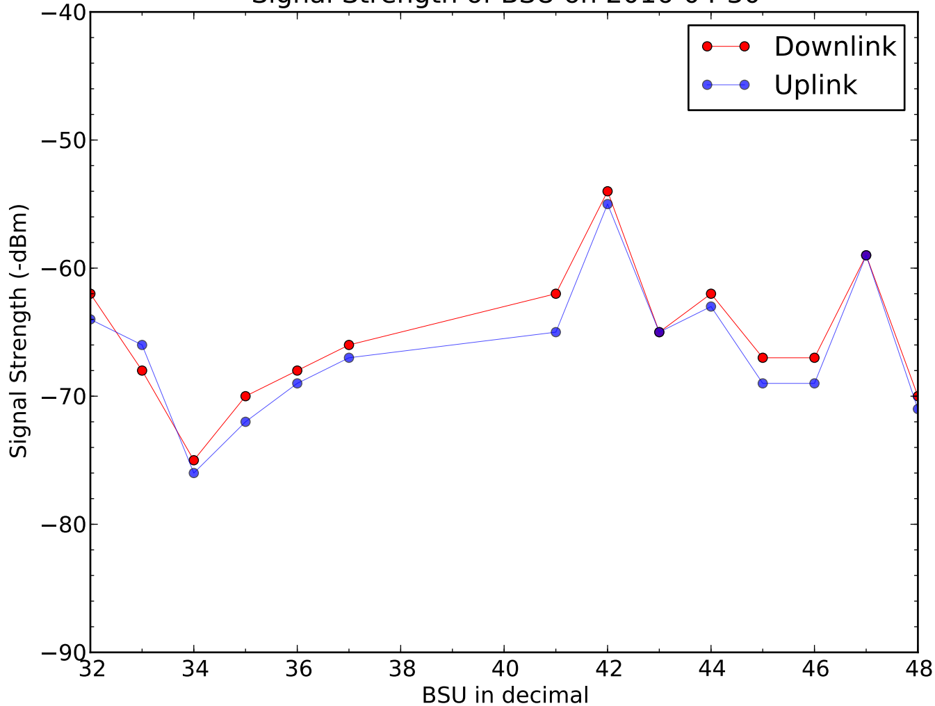
Signal Strength of BSU on 2016-04-30
