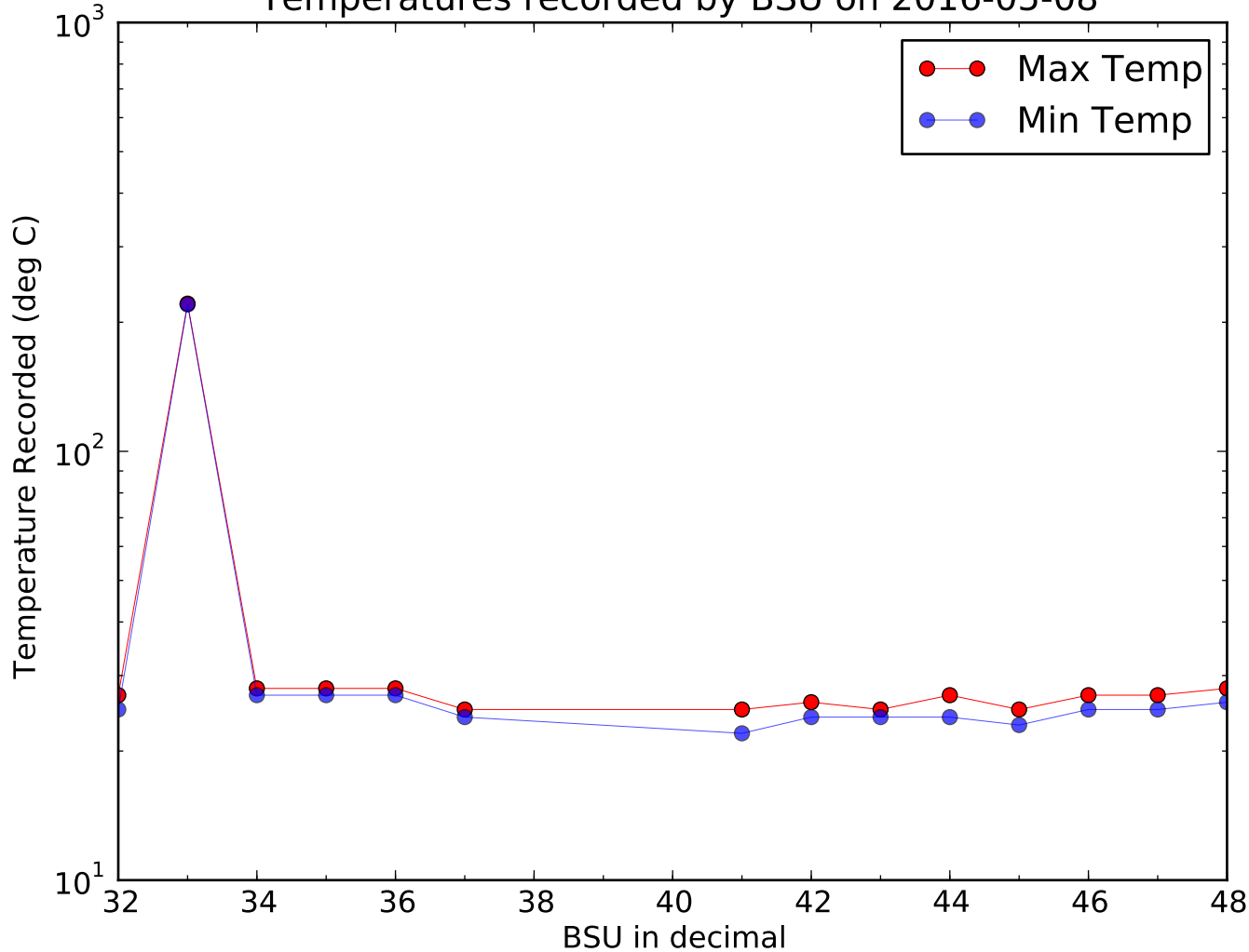
Temperatures recorded by BSU on 2016-05-08
