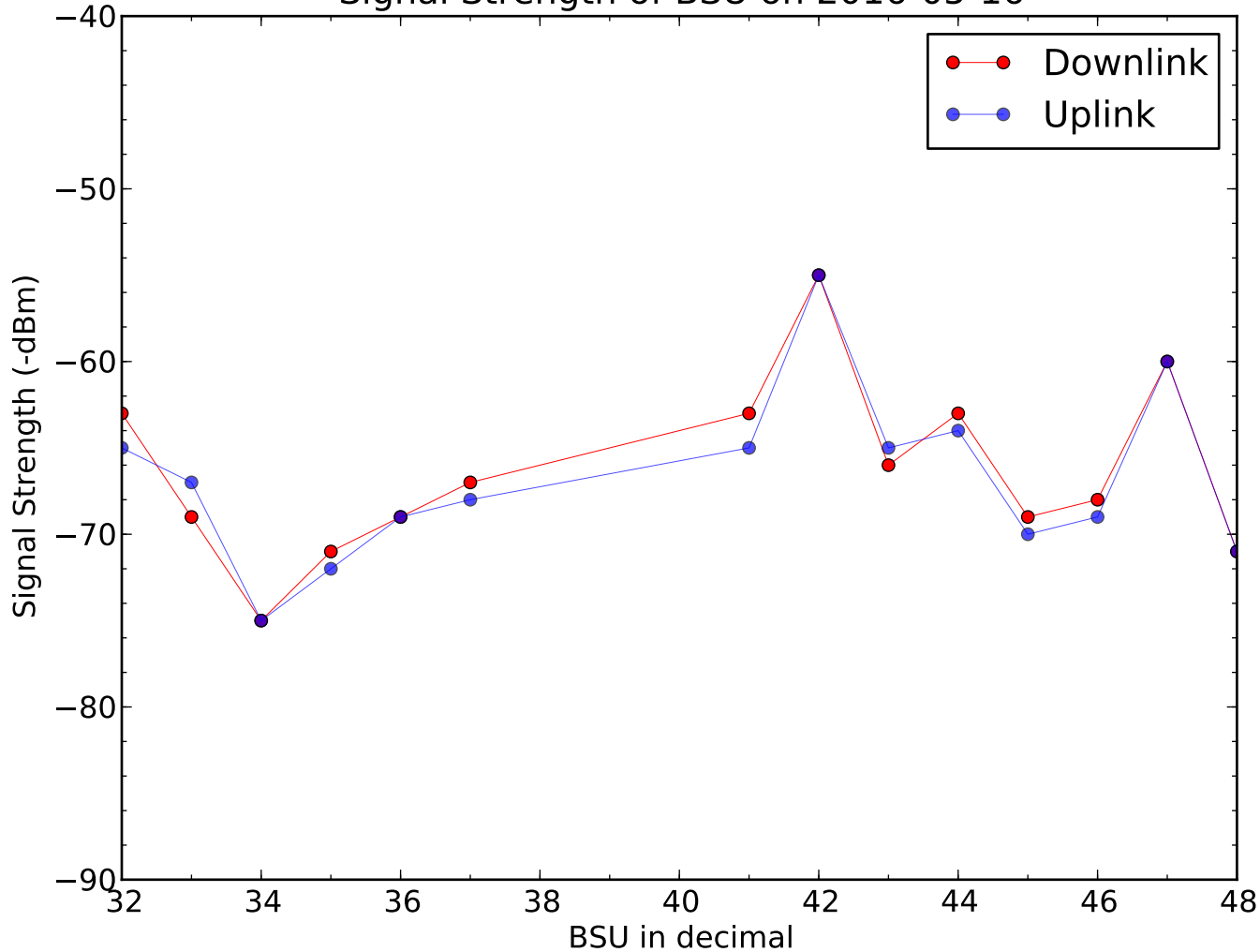
Signal Strength of BSU on 2016-05-16
