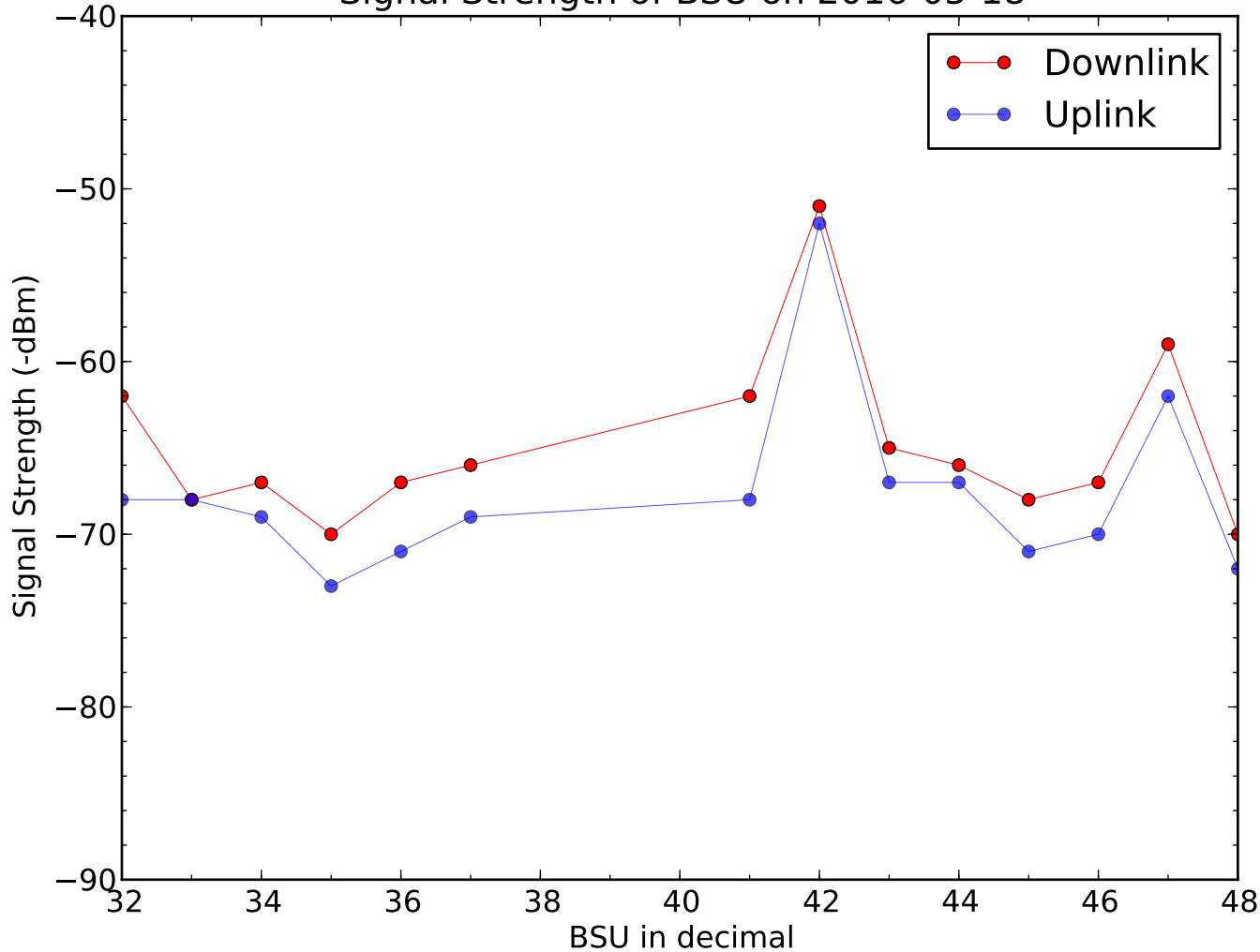
Signal Strength of BSU on 2016-05-18
