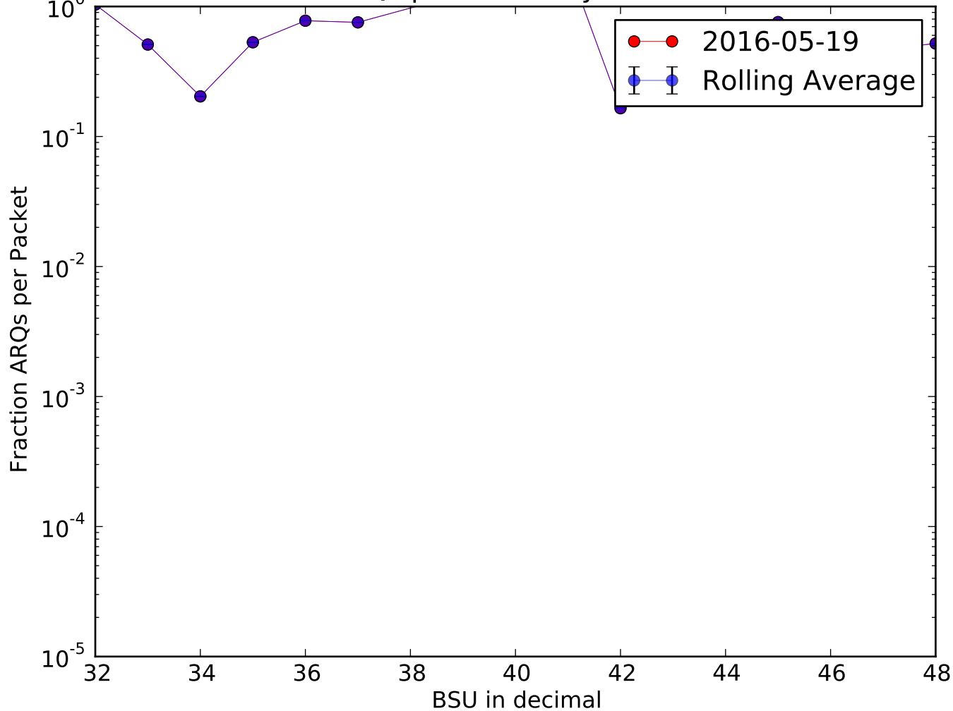
Fraction ARQs per Packet by BSU 2016-05-19
