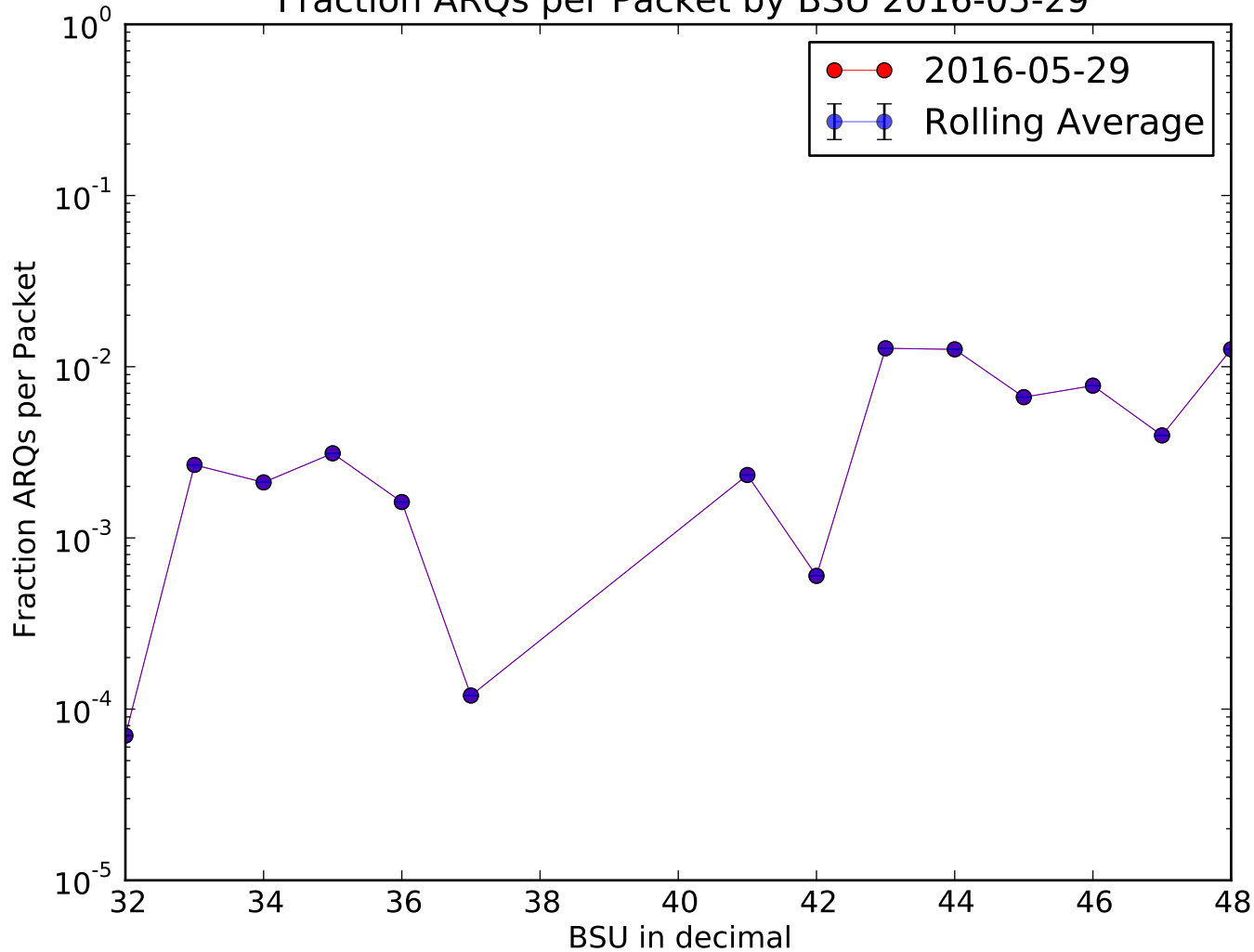
Fraction ARQs per Packet by BSU 2016-05-29
