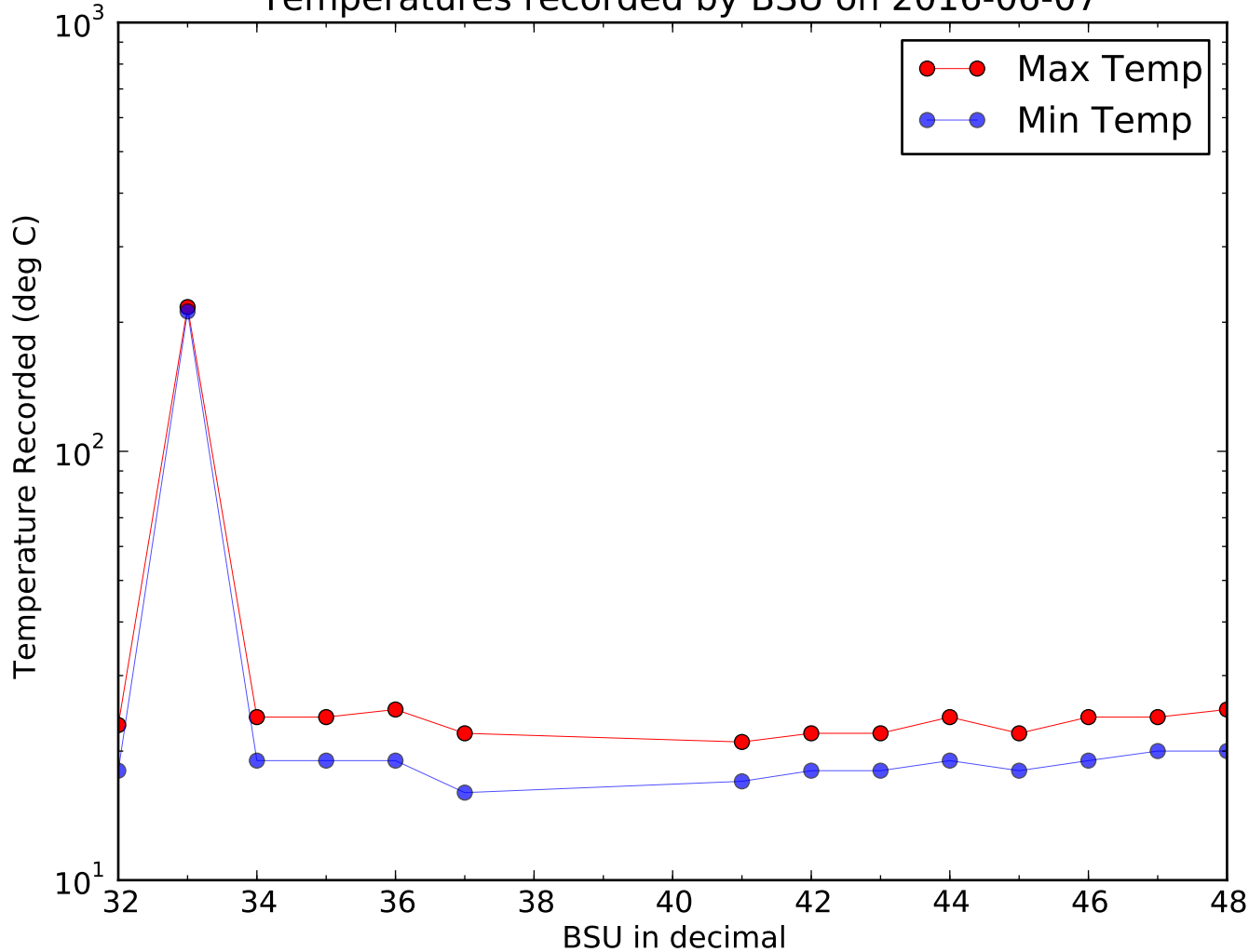
Temperatures recorded by BSU on 2016-06-07
