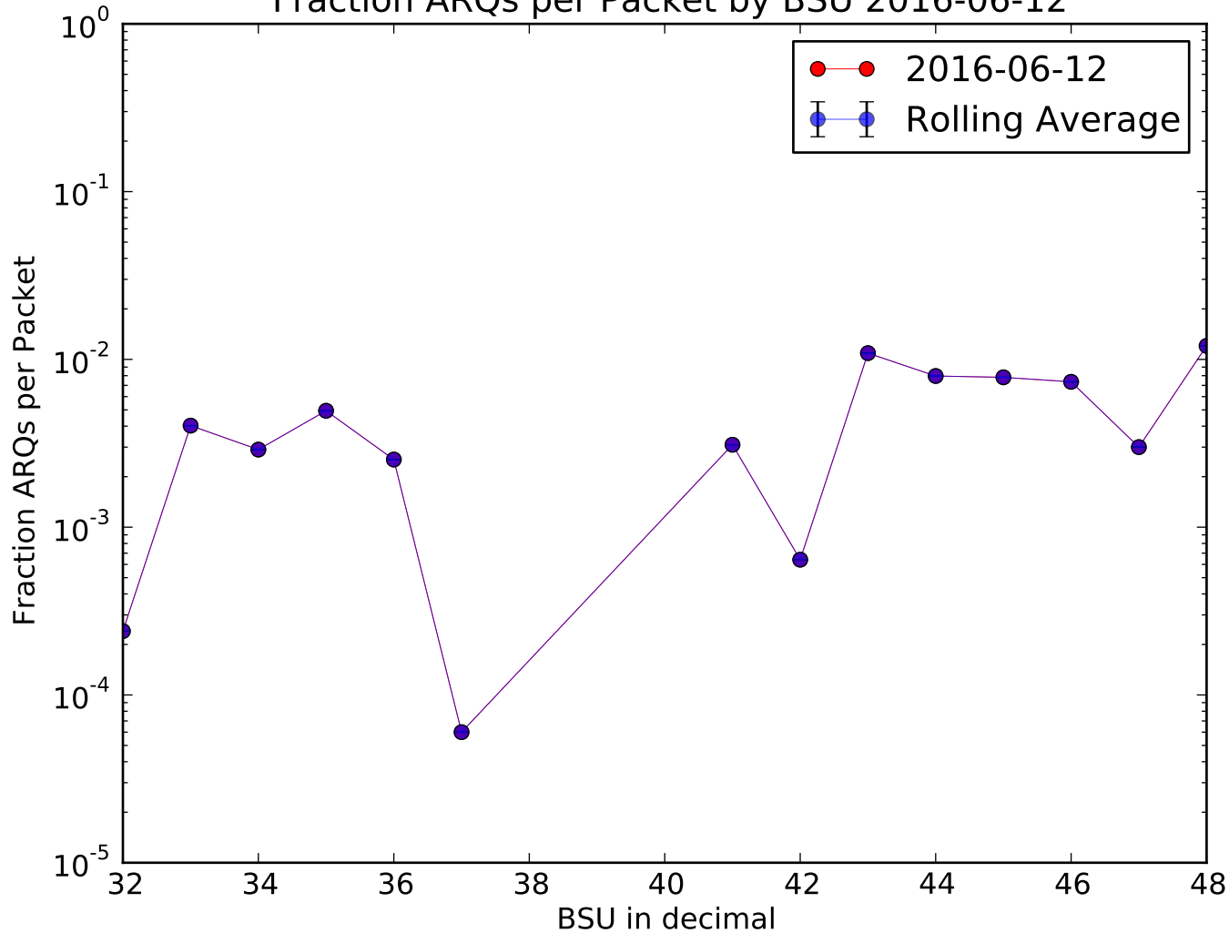
Fraction ARQs per Packet by BSU 2016-06-12
