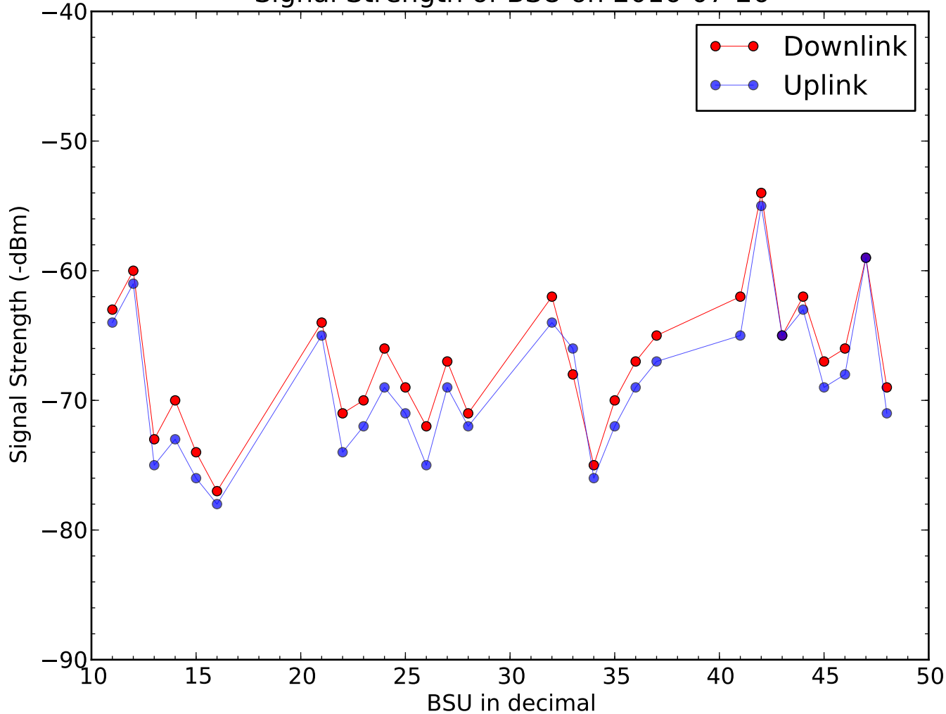
Signal Strength of BSU on 2016-07-26
