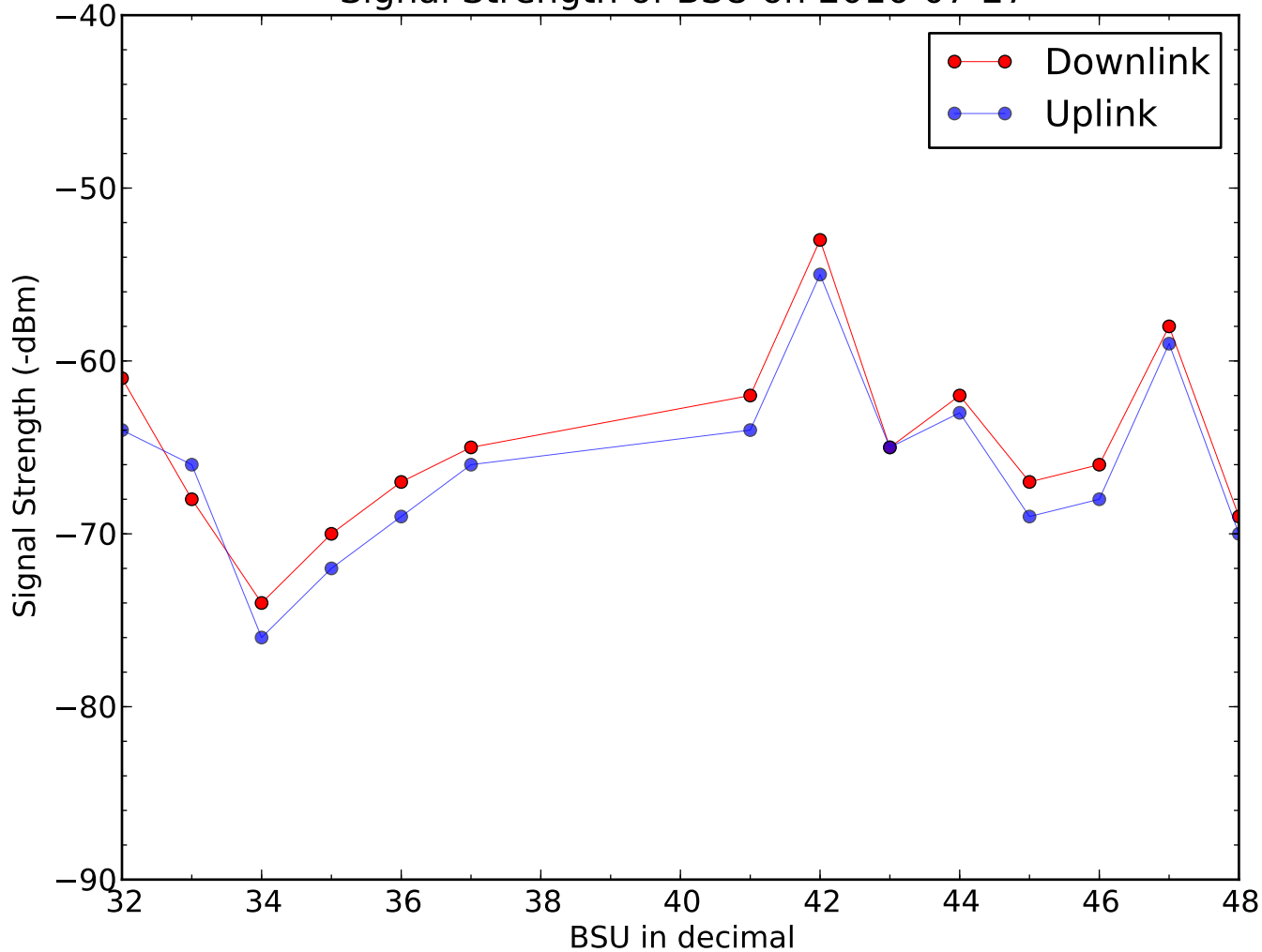
Signal Strength of BSU on 2016-07-27
